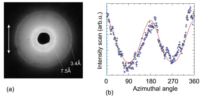
FIG. 3. (Color online) (a) The x-ray scattering image showing key reflections; the outer ring ( 3.4 \text{ \AA} ) is the signal from the multi-wall nanotubes. The inner ring ( 7.5 \text{ \AA} ) represents the PDMS mesh size; see Sec. III B. The arrow shows the direction of the uniaxial aligning strain. (b) The typical azimuthal intensity variation I(\beta) at a scattering angle of 3.4 \text{ \AA} reflection. The data are fitted by the model Ref. 29.
