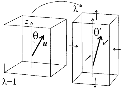
FIG. 6. The scheme of an affine incompressible extension, changing the orientation of an inflexible rod embedded in the medium.
