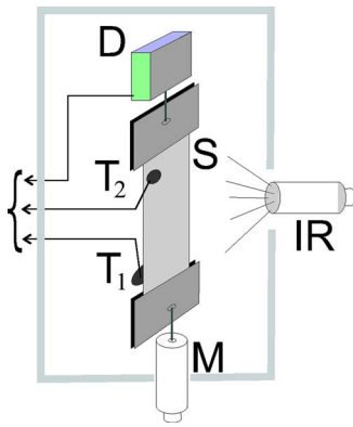
FIG. 1. (Color online) Scheme of the apparatus; see text for detail.
