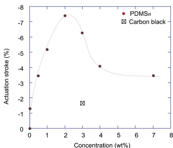
FIG. 11. (Color online) The magnitude of the actuation stroke at \varepsilon=40\% as a function of filler concentration n . The maximum of the response at \sim 2 wt % is evident. The single square symbol gives the value for 3 wt % carbon black filler in PDMS.
