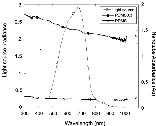
FIG. 2. Spectral data of the light source (left axis, arbitrary units), and the normalized absorption of the PDMS0.3 composite and the control pristine PDMS elastomer (right axis).
