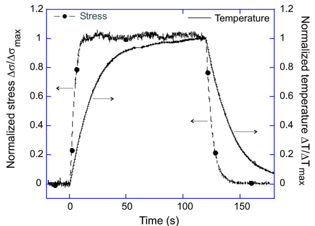
FIG. 9. (Color online) The normalized stress response plotted alongside the normalized change in temperature, as functions of time (PDMS3, prestrain \epsilon=20\% ); see text for discussion.
