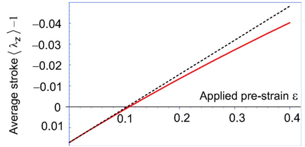
FIG. 14. (Color online) The result of the affine theoretical model, Eq. (10); the dashed line shows the linear approximation at small prestrain. The nanotube contraction factor is chosen to be \Delta = 0.8 , as suggested by the crossover strain value \varepsilon^* \sim 0.1 .
