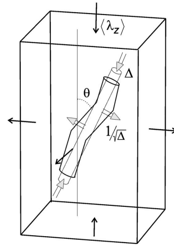
FIG. 13. The scheme illustrating how the distortion (kinking) of an individual tube, lying at an angle \theta to the macroscopic alignment axis, projects on the z axis to contribute to the average uniaxial strain, Eq. (10).
