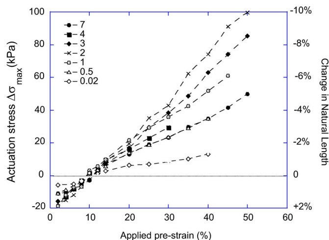
FIG. 10. (Color online) The magnitude (in kPa) of exerted actuation stress (the height of steps in Fig. 7, \Delta\sigma_{\max} ), as a function of prestrain. Different PDMS composites are labeled on the plot by their wt % value. The right y axis shows the corresponding actuation stroke: the change in natural length L_0(\text{IR}) .
