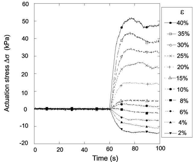
FIG. 8. The speed of actuation response, illustrated by plotting the actuation stress in PDMS3 nanocomposite, \Delta\sigma in kPa, as a function of time for different prestrain values (labeled on the plot).
