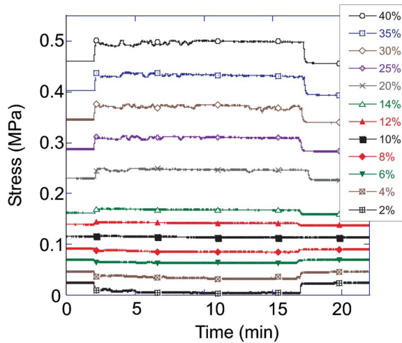
FIG. 7. (Color online) The response of a 1 wt % nanocomposite PDMS1 to IR radiation at different levels of prestrain \epsilon . Stress is measured at fixed sample length (different prestrain curves labeled on the plot).
