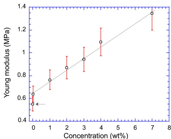
FIG. 4. (Color online) Young modulus Y for PDMS nanocomposites at increasing MWCNT loading. The arrow points at the value for control PDMS rubber.
