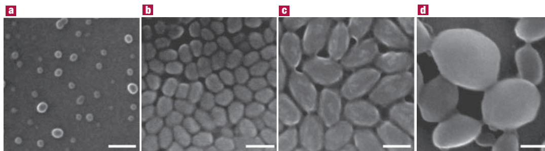
Figure 5 SEM images of PFO nanoparticles with different shapes and sizes. a–c , The aspect ratios of (a) spheres (25 nm), (b) ellipsoids and (c) ellipsoids are 1.0, 1.45 and 1.8 respectively. d , The nanoparticles are irregular in shape when the size is over 200 nm. The white bar represents 100 nm.
