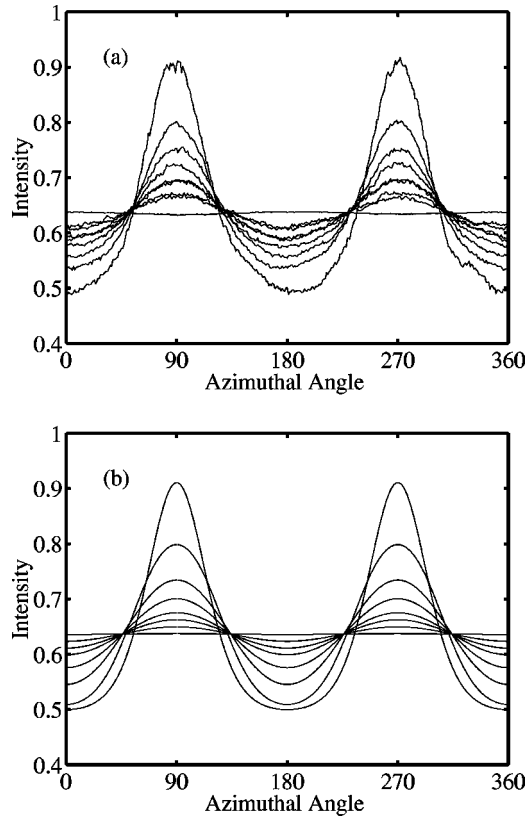
FIG. 6. (a) Azimuthal intensity (arb. units) distribution around the wide-angle diffraction ring for \lambda_{xx} = 1.00, 1.04, 1.08, 1.12, 1.16, 1.24, 1.32 , and 1.40 . At \lambda_{xx} = 1.00 , the profile is flat to within our experimental error. The scattering profile showing the highest dependence of intensity on azimuthal angle is obtained from a nematic liquid crystal elastomer. (b) Theoretical prediction from Eq. (3.1) for the same strain values as (a).
