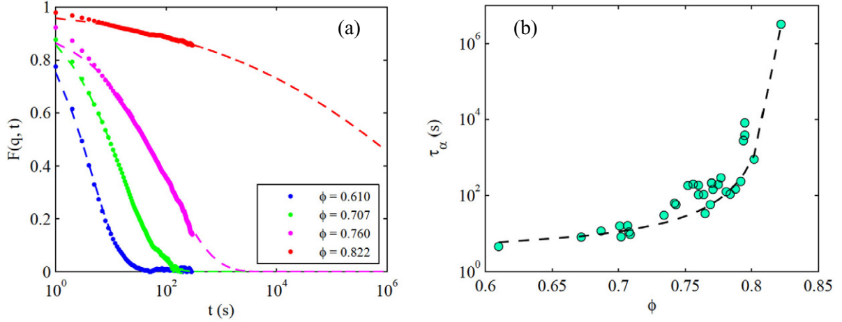
Figure 2. The system relaxation time can be obtained for most samples. (a) Intermediate scattering function versus time for four representative samples: \phi = 0.610 and s = 10\% ; \phi = 0.707 and s = 11\% ; \phi = 0.760 and s = 11\% ; \phi = 0.822 and s = 11\% . Experimental data are fitted with F(q, t) = C \exp[-(t/\tau_\alpha)^\beta] (dashed lines). (b) System relaxation time \tau_\alpha , obtained from the fit of F(q, t) , versus the area fraction \phi . The dashed line is a fit according to the Vogel–Fulcher–Tamman form equation (4).
